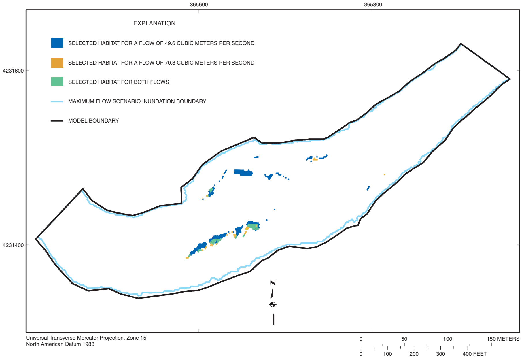
Figure 4-85. Selected habitat area distribution for habitat category 20 (flathead catfish) at flows of 49.6 and 70.8 cubic meters per second at Marais des Cygnes River site MDC2.
